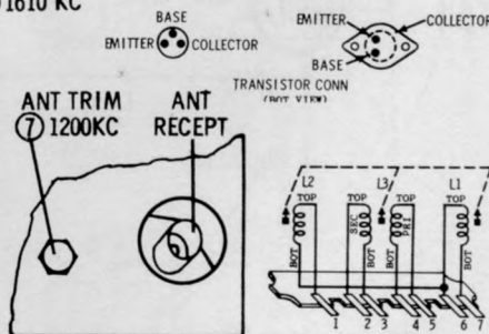
BACK VIEW
